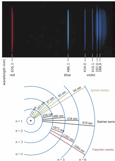
Visible spectrum of hydrogen in Balmer series
