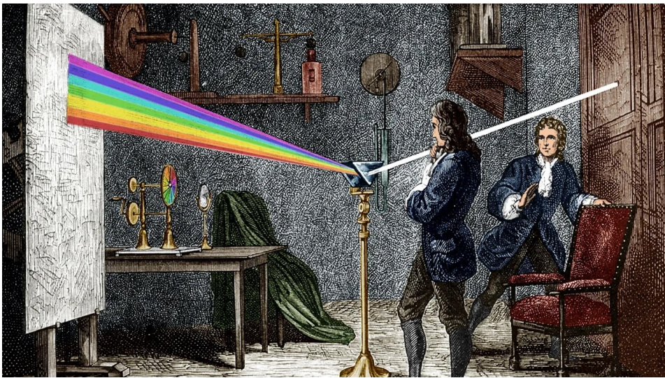
Newton beams white light through prism in Trinity College 1666
